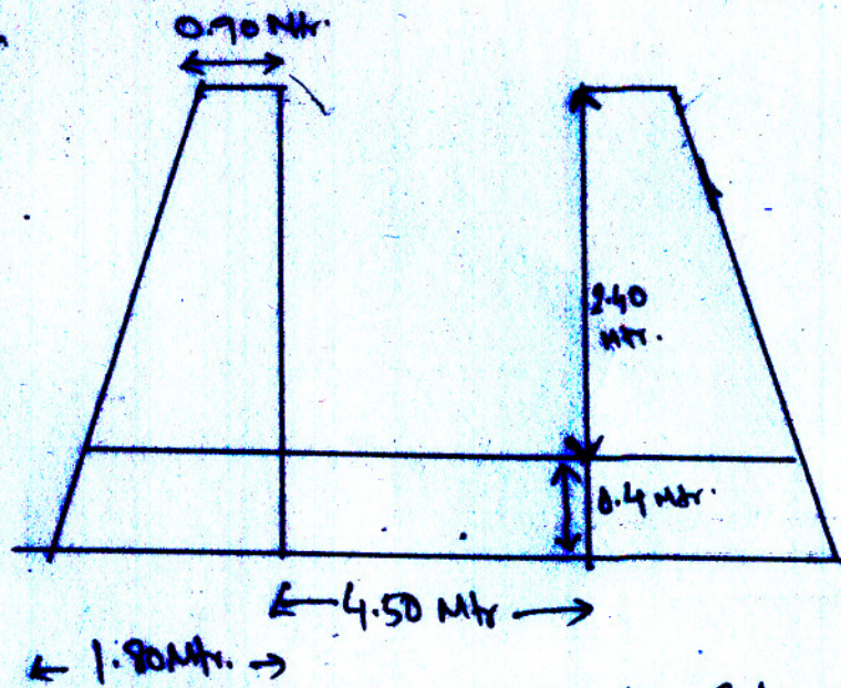
FRONT ELEVATION & C/S OF GATE
