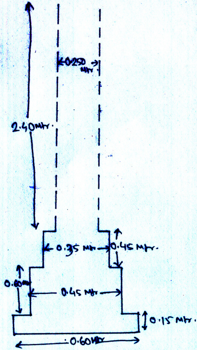
C/S OF BOUNDARY WALL
